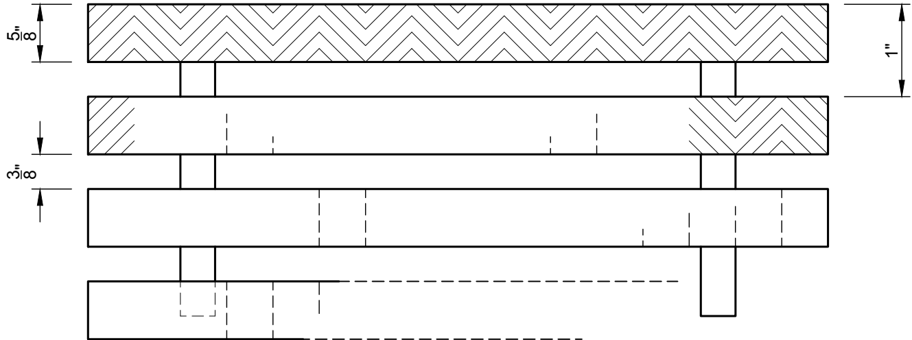
Top View
